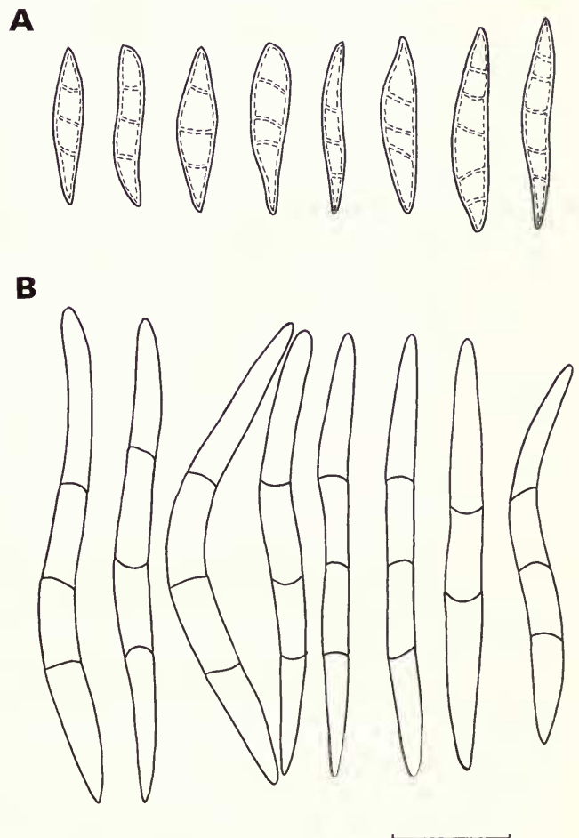
Fig. 69. Ascospore outlines (A) Verrucaria byssacea var. minutissima Ach. (BM-ACH 312-isotype); (B) Lahmiomyces piceae (Anzi) Tom. & Cif. (BM-isotype of Lahmia piceae ); scale = 10 µm.
